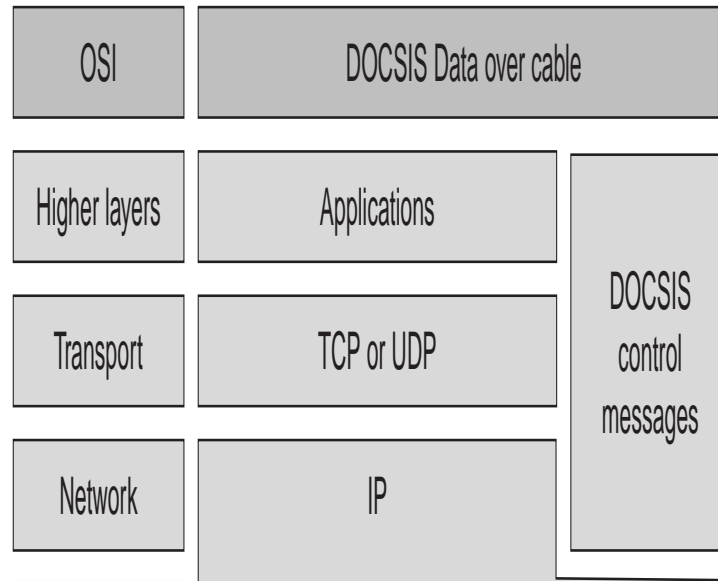
Figure 22-4 DOCSIS and OSI Protocol Layers
