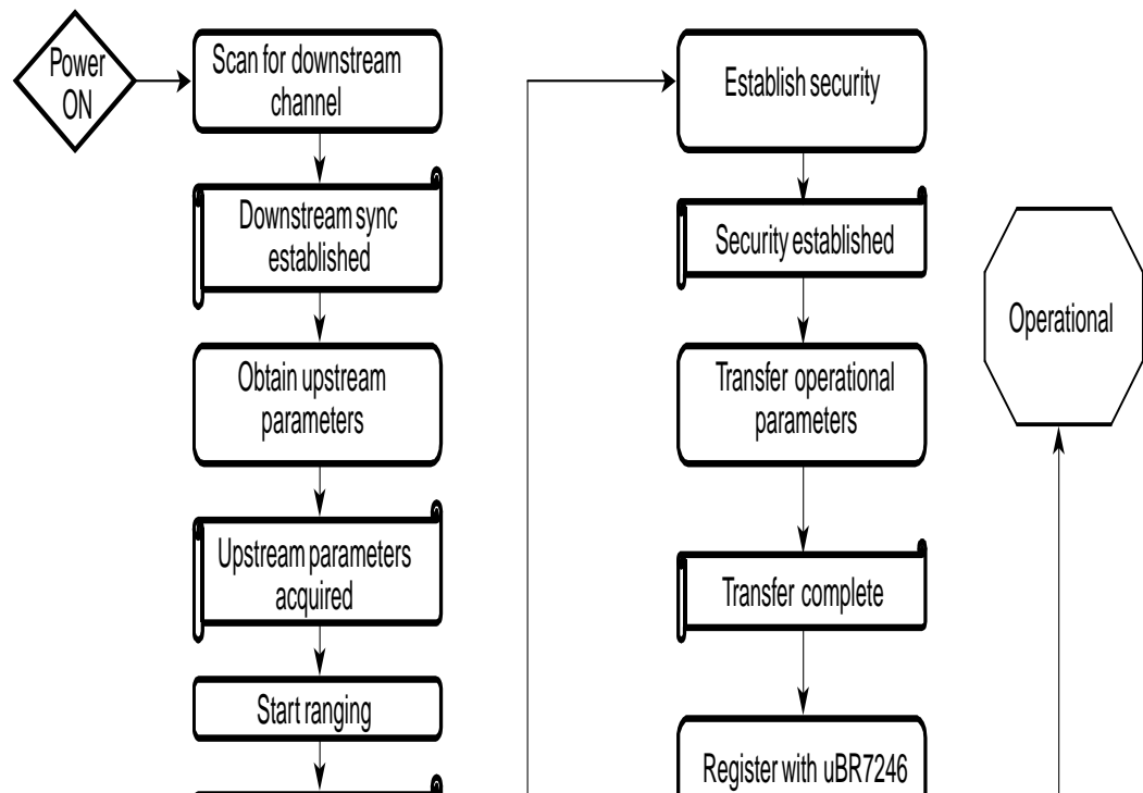
Figure 22-5 Cable Modem Registration Sequence
